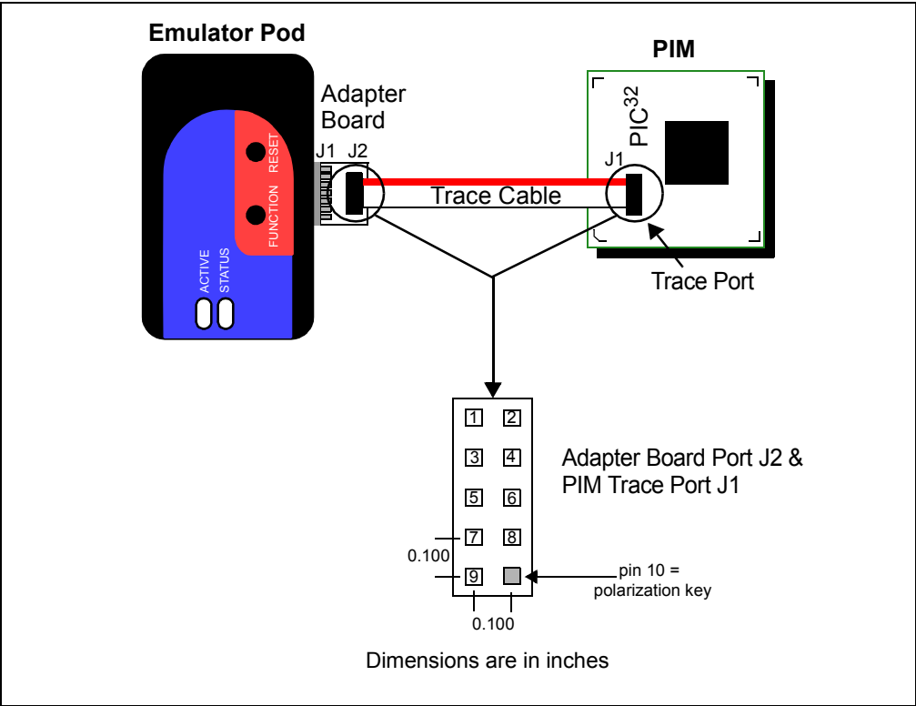
FIGURE 17-4: TRACE INTERFACE CONNECTIONS WITH A PIM
