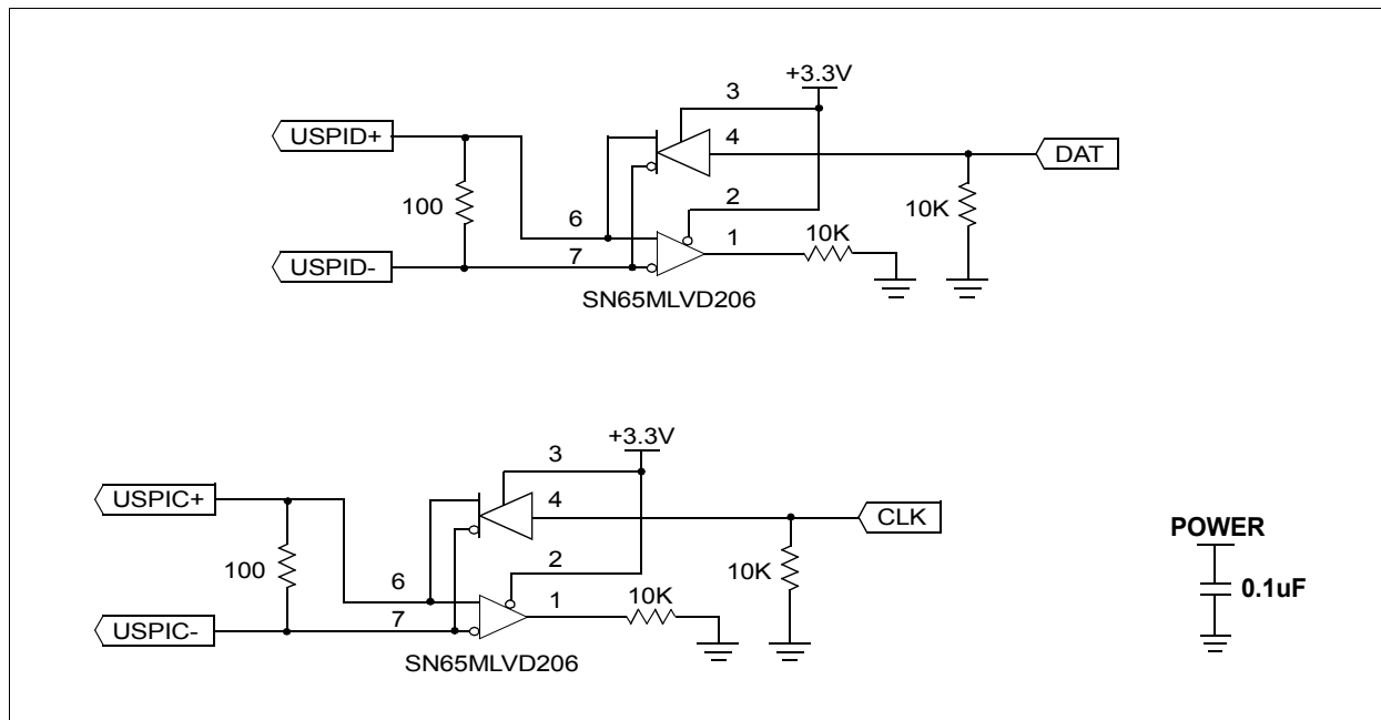
FIGURE 14-6: RECEIVER BOARD SCHEMATIC – DAT & CLK
