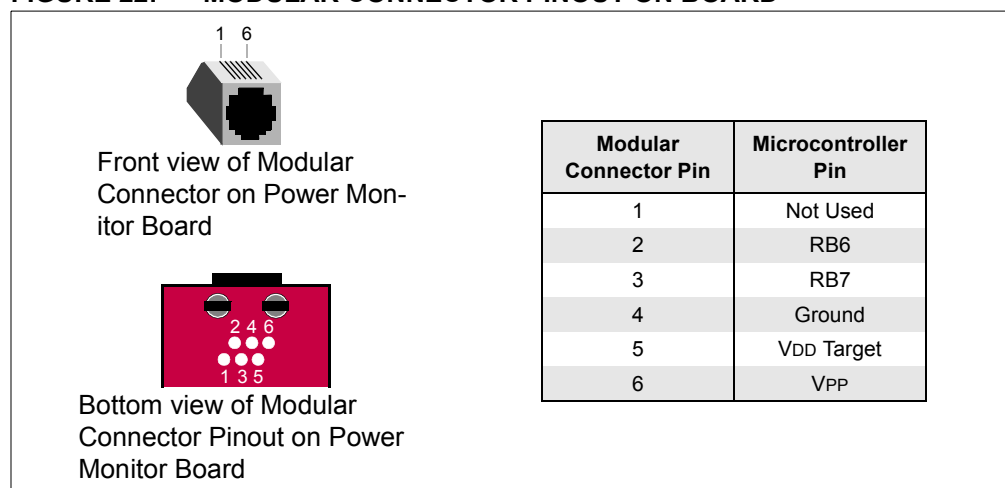
FIGURE 22: MODULAR CONNECTOR PINOUT ON BOARD
