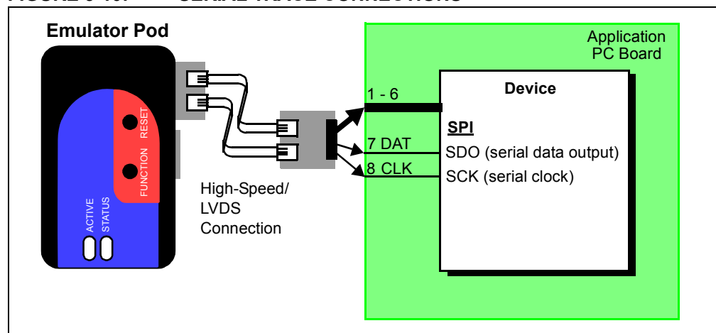
FIGURE 3-10: SERIAL TRACE CONNECTIONS
