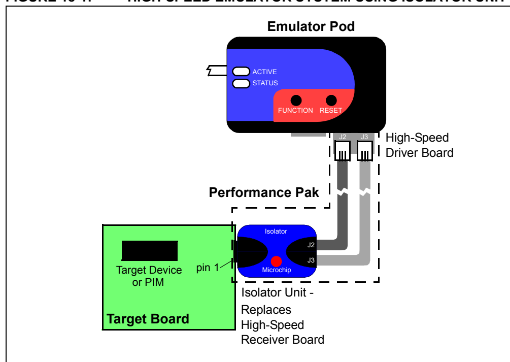
FIGURE 18-1: HIGH-SPEED EMULATOR SYSTEM USING ISOLATOR UNIT
