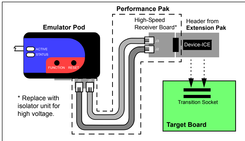
FIGURE 3-5: HIGH-SPEED/LVDS CONNECTION – ICE DEVICE
