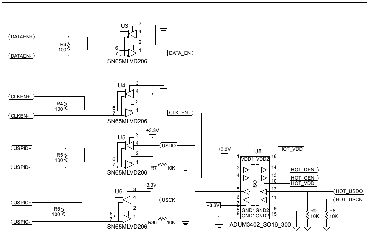
FIGURE 18-4: ISOLATOR UNIT SCHEMATIC - DAT & CLK
