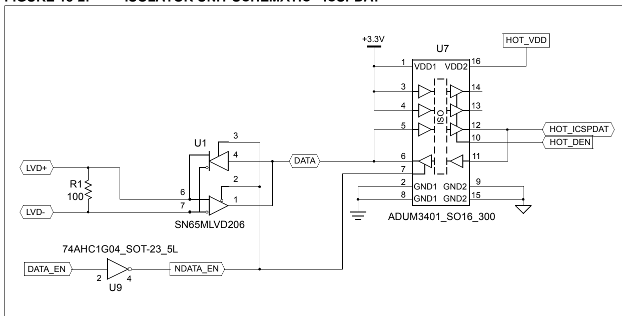
FIGURE 18-2: ISOLATOR UNIT SCHEMATIC - ICSPDAT
