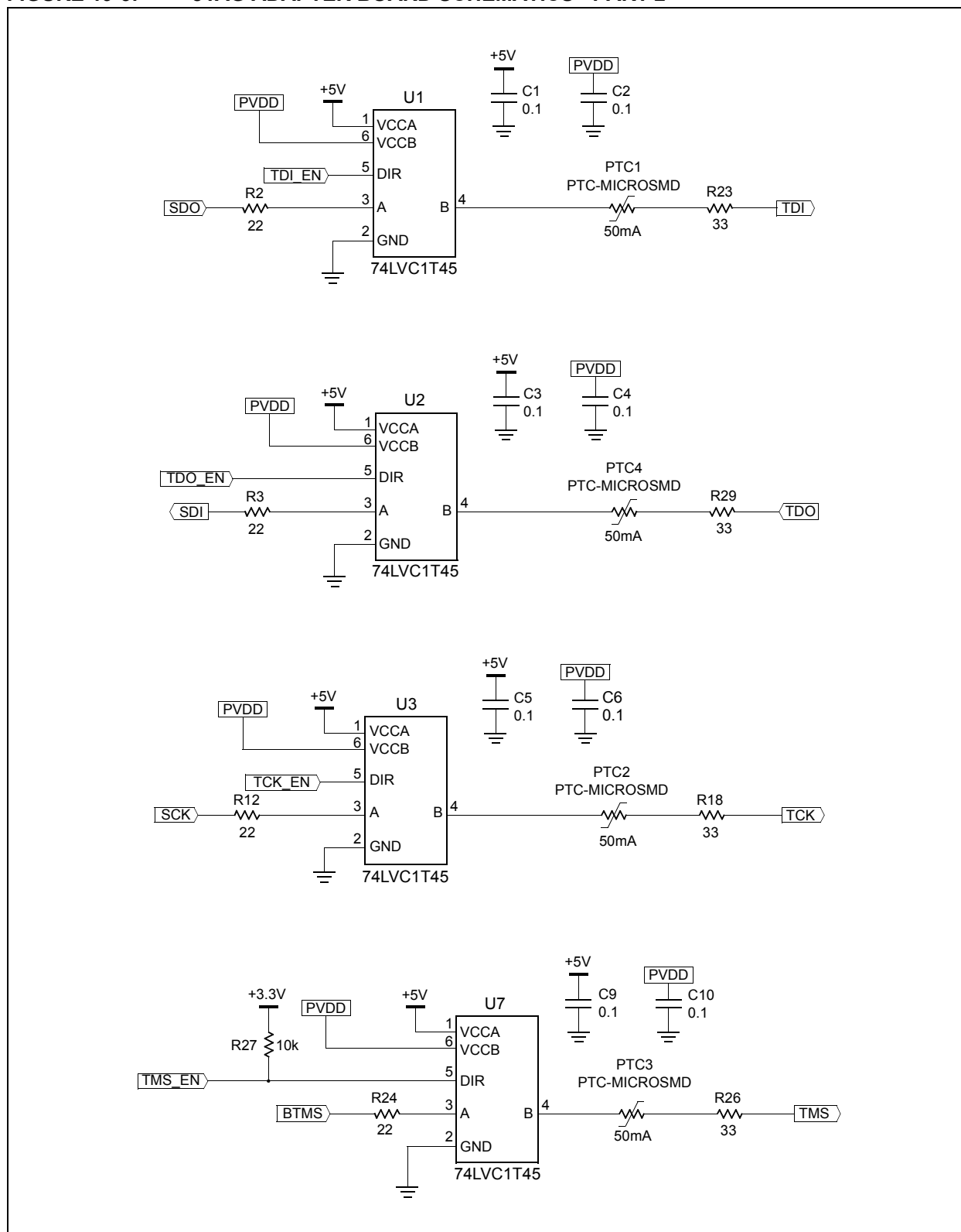
FIGURE 19-3: JTAG ADAPTER BOARD SCHEMATICS - PART 2
