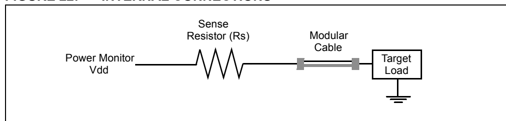
FIGURE 22: INTERNAL CONNECTIONS
