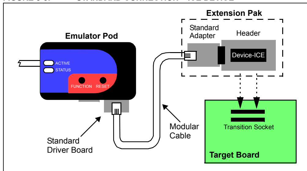
FIGURE 3-3: STANDARD CONNECTION – ICE DEVICE
