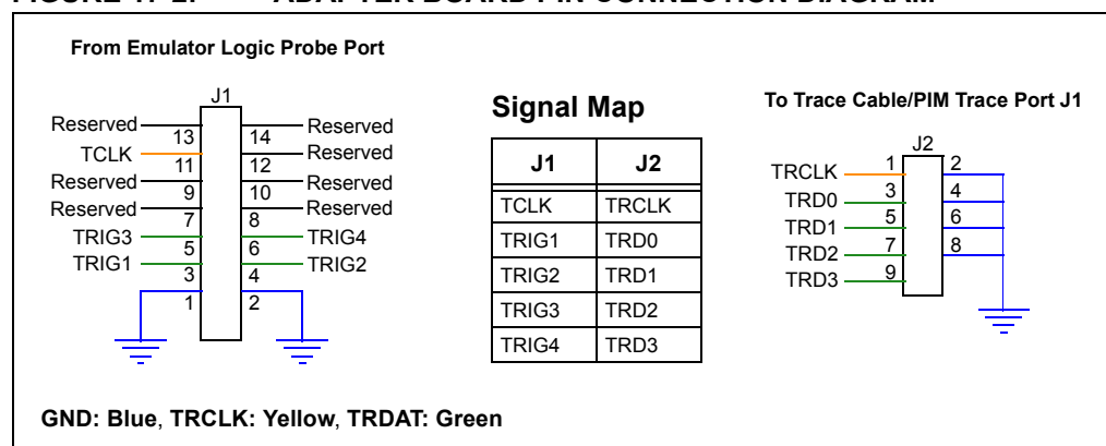
FIGURE 17-2: ADAPTER BOARD PIN CONNECTION DIAGRAM
