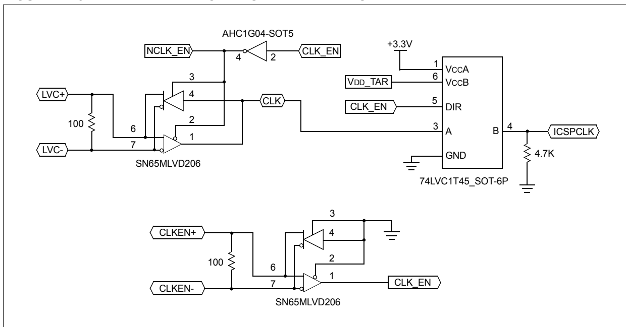
FIGURE 14-5: RECEIVER BOARD SCHEMATIC – ICSPCLK
