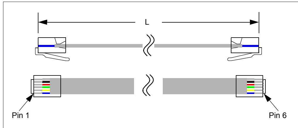
FIGURE 13-3: MODULAR CABLE
