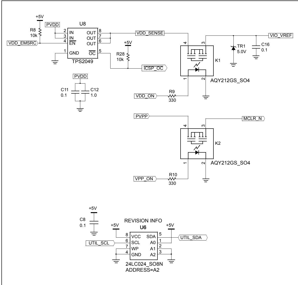
FIGURE 19-4: JTAG ADAPTER BOARD SCHEMATICS - PART 3
