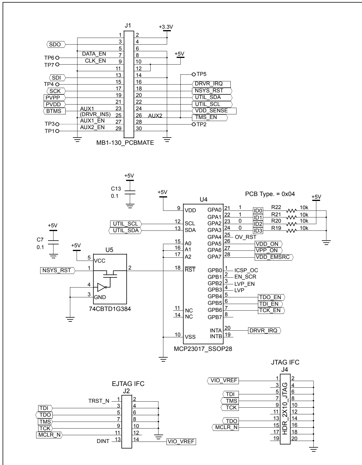
FIGURE 19-2: JTAG ADAPTER BOARD SCHEMATICS - PART 1
