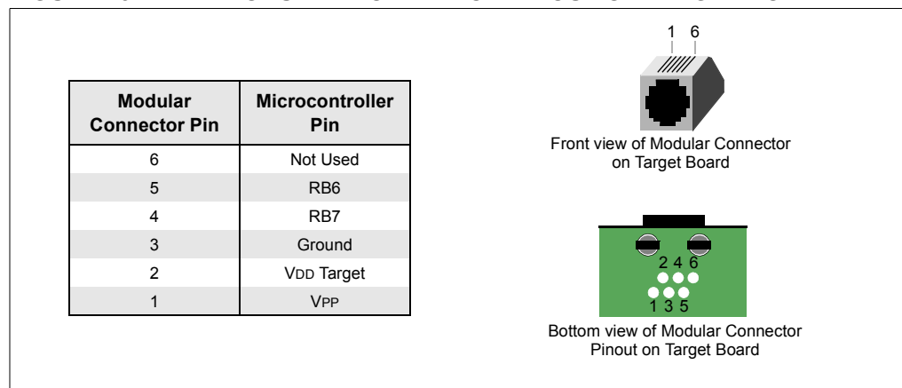
FIGURE 13-4: MODULAR CONNECTOR PINOUT OF TARGET BOARD
