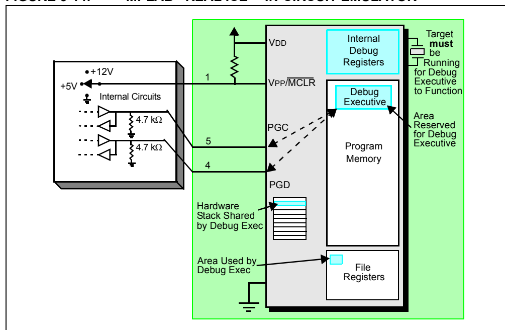
FIGURE 3-14: MPLAB® REAL ICE™ IN-CIRCUIT EMULATOR
