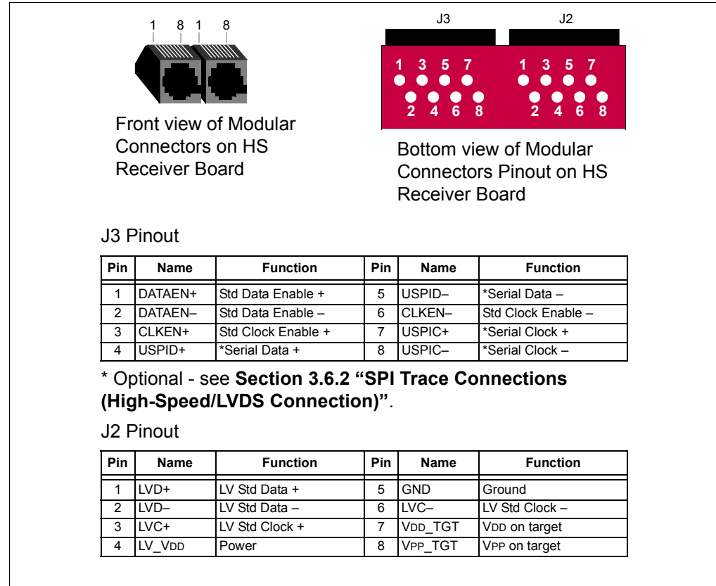
FIGURE 14-2: MODULAR CONNECTORS PINOUT OF HIGH-SPEED RECEIVER BOARD
