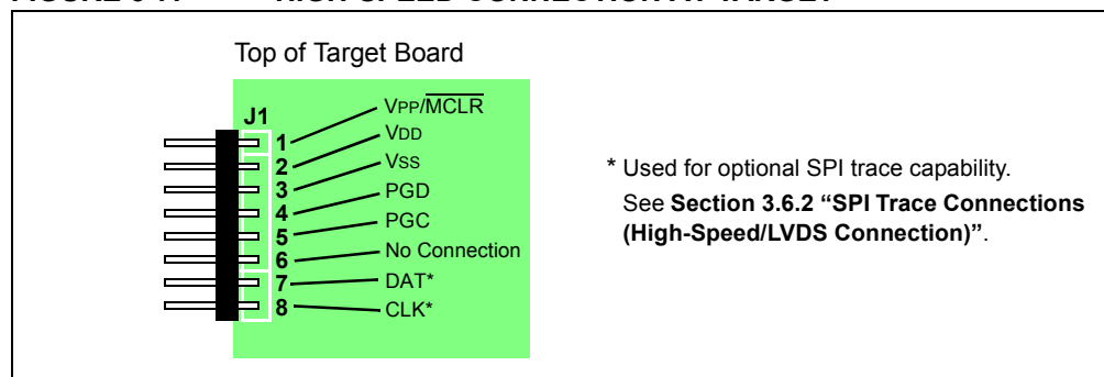
FIGURE 3-7: HIGH-SPEED CONNECTION AT TARGET
