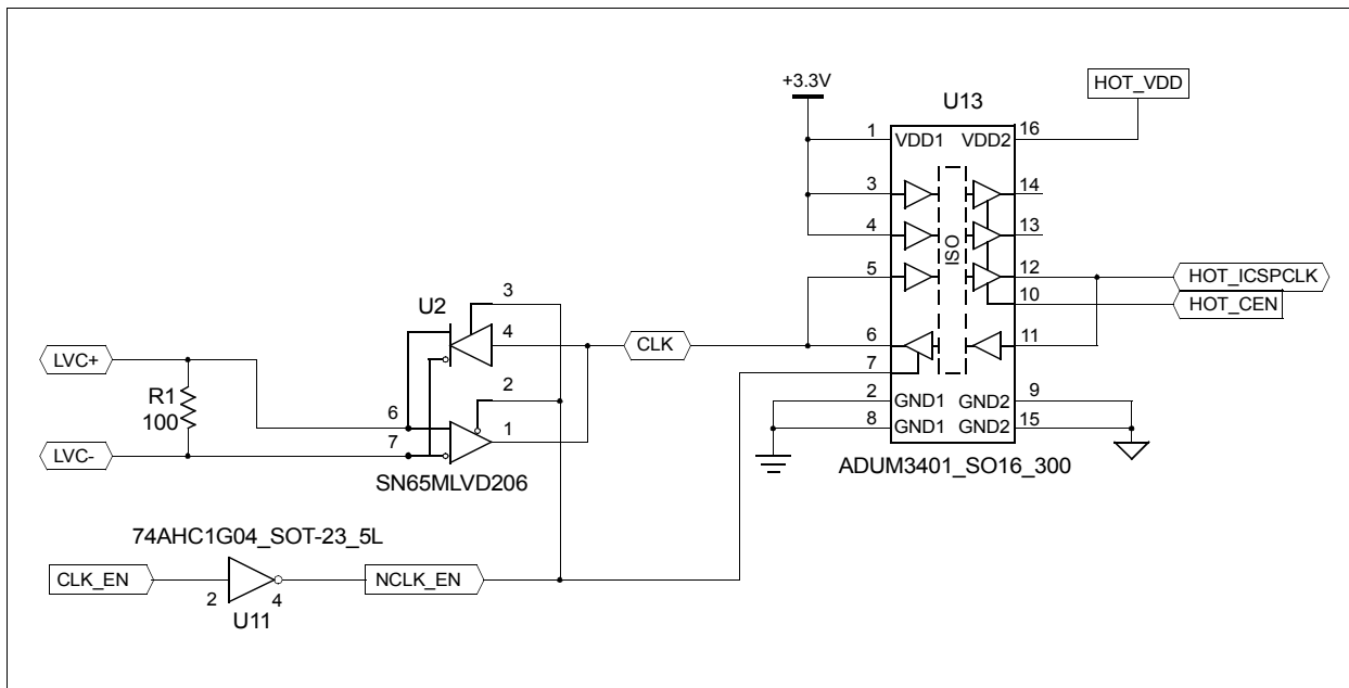
FIGURE 18-3: ISOLATOR UNIT SCHEMATIC - ICSPCLK
