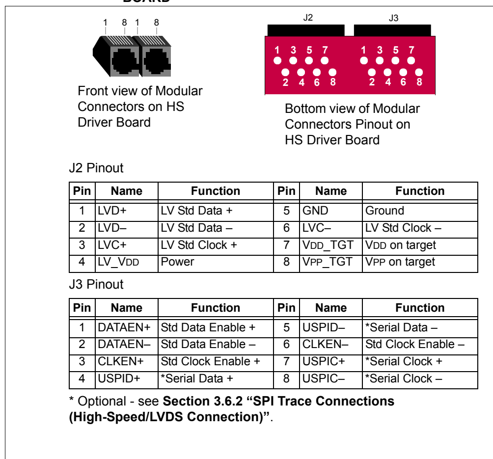
FIGURE 14-1: MODULAR CONNECTORS PINOUT OF HIGH-SPEED DRIVER BOARD
