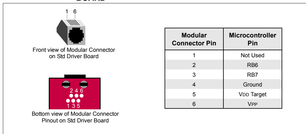
FIGURE 13-2: MODULAR CONNECTOR PINOUT OF STANDARD DRIVER BOARD
