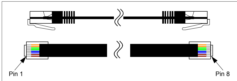
FIGURE 14-7: LVDS CABLE
