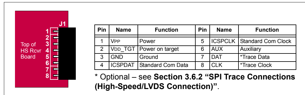
FIGURE 14-3: 8-PIN HEADER PINOUT OF HIGH-SPEED RECEIVER BOARD
