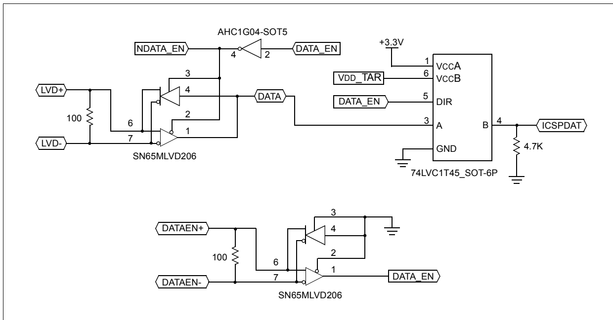
FIGURE 14-4: RECEIVER BOARD SCHEMATIC – ICSPDAT
