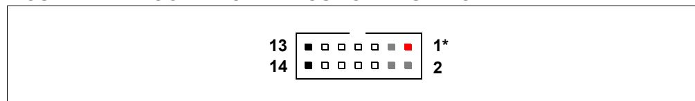
FIGURE 21: LOGIC PROBE PINOUT ON EMULATOR
