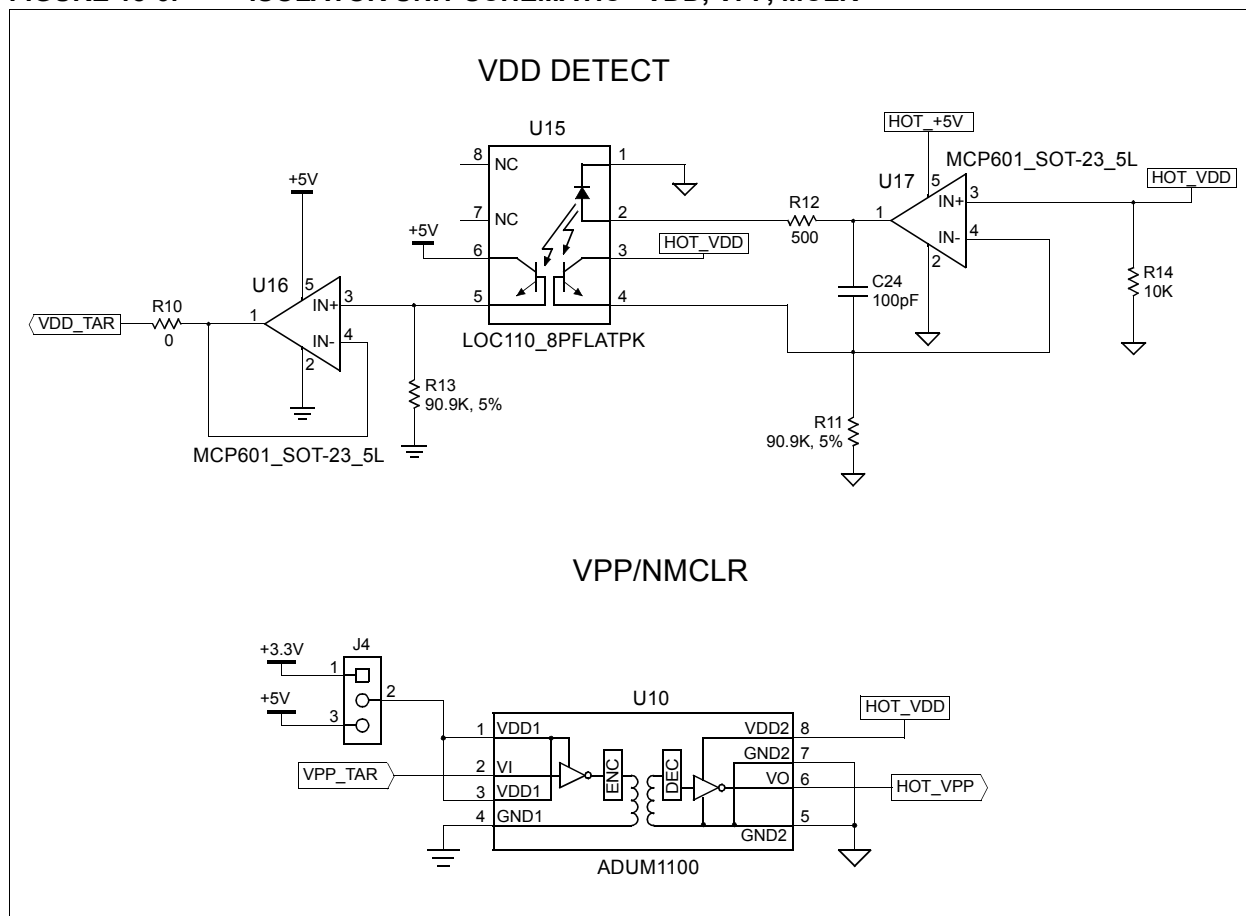
FIGURE 18-6: ISOLATOR UNIT SCHEMATIC - VDD, VPP, MCLR
