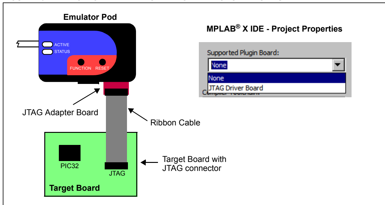
FIGURE 19-1: JTAG ADAPTER BOARD CONNECTIONS AND SET UP
