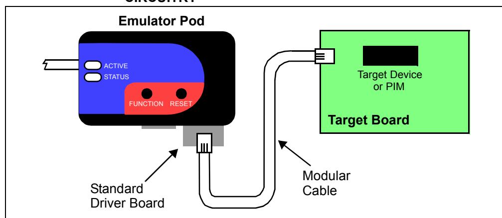
FIGURE 3-2: STANDARD CONNECTION – DEVICE WITH ON-BOARD ICE CIRCUITRY
