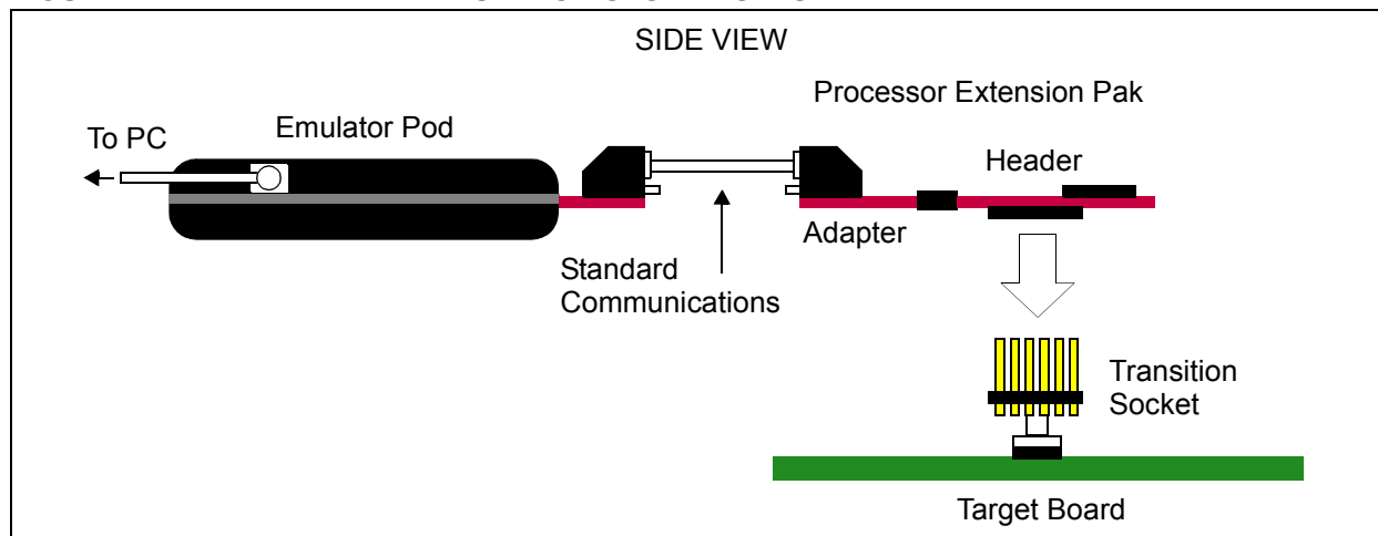
FIGURE 1-1: EXAMPLE EMULATOR SYSTEM SETUP
