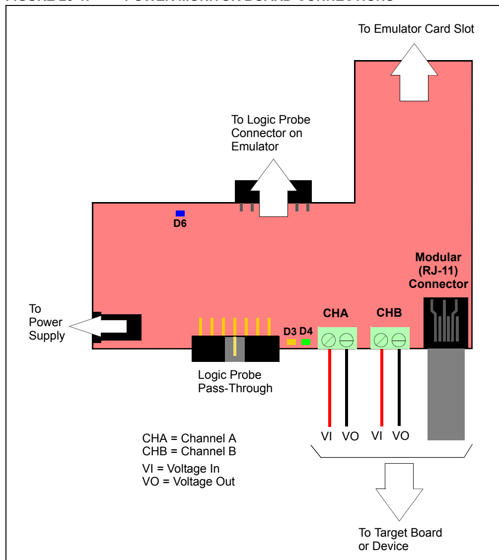
FIGURE 20-1: POWER MONITOR BOARD CONNECTIONS
