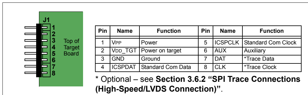
FIGURE 14-8: 8-PIN HEADER PINOUT AT TARGET
