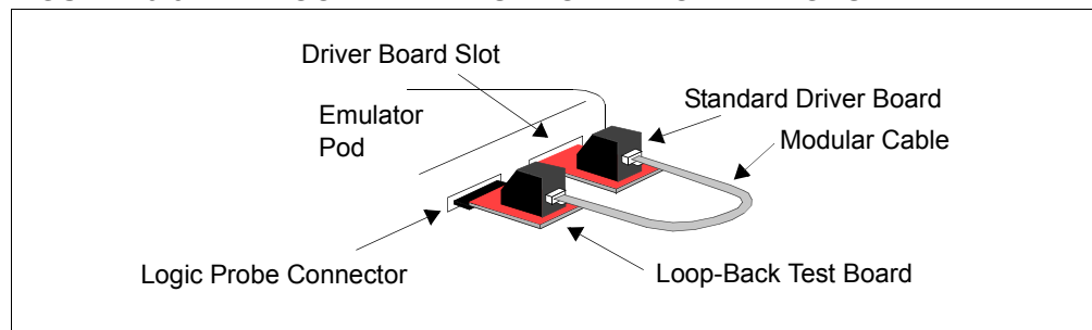
FIGURE 13-5: LOOP-BACK TEST BOARD CONNECTIONS
