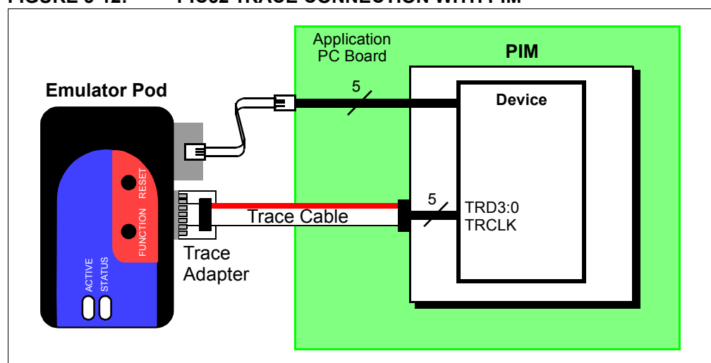
FIGURE 3-12: PIC32 TRACE CONNECTION WITH PIM
