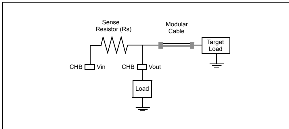
FIGURE 25: CHB INTERNAL CONNECTIONS
