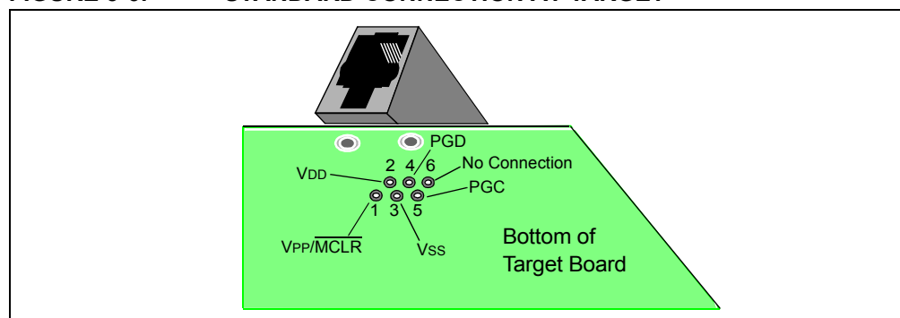
FIGURE 3-6: STANDARD CONNECTION AT TARGET
