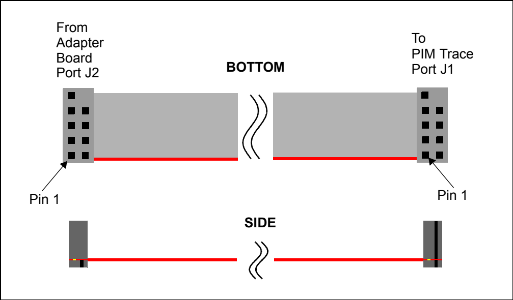
FIGURE 17-3: TRACE CABLE DIAGRAM
