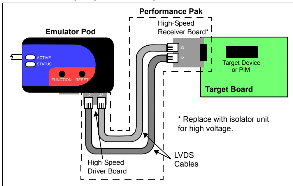
FIGURE 3-4: HIGH-SPEED/LVDS CONNECTION – DEVICE WITH ON-BOARD ICE CIRCUITRY
