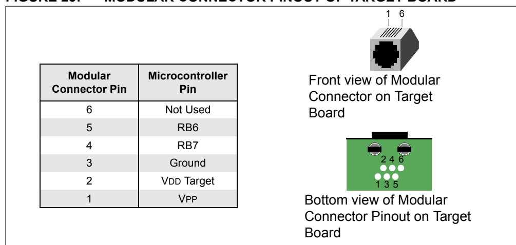
FIGURE 23: MODULAR CONNECTOR PINOUT OF TARGET BOARD
