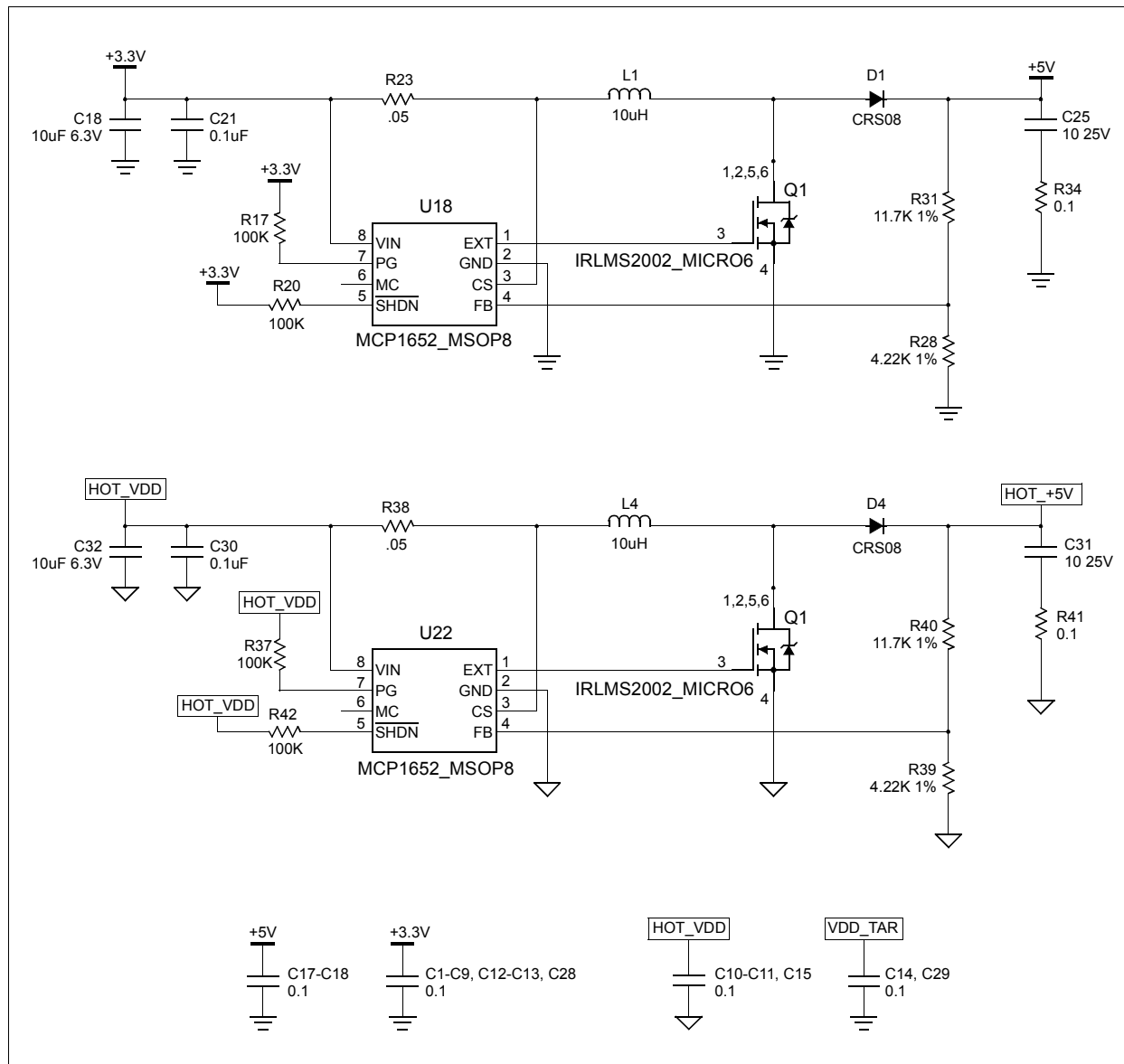
FIGURE 18-5: ISOLATOR UNIT SCHEMATIC - POWER
