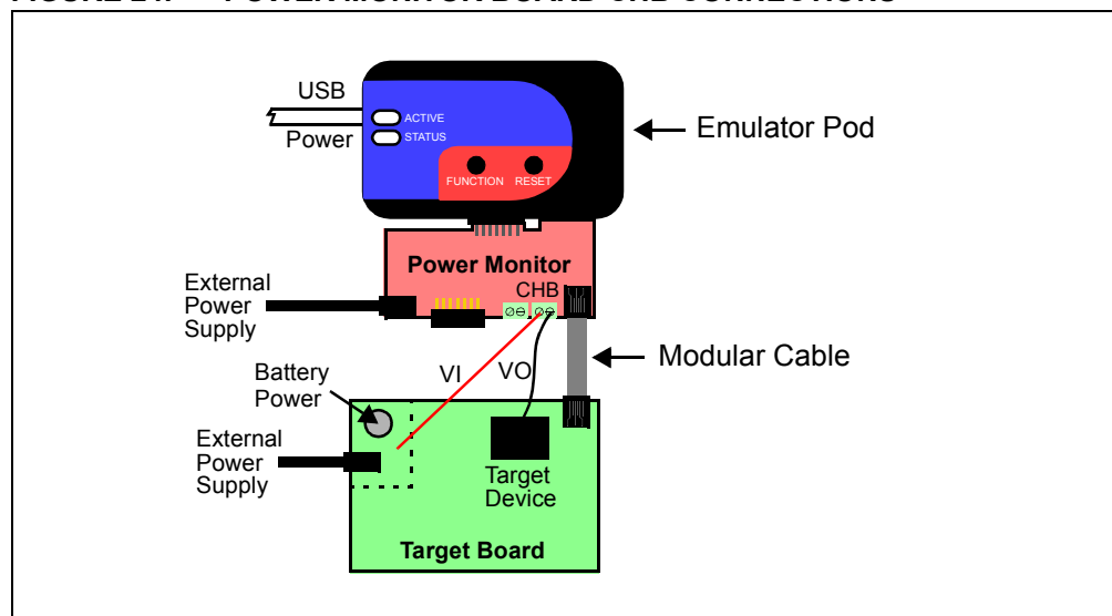
FIGURE 24: POWER MONITOR BOARD CHB CONNECTIONS
