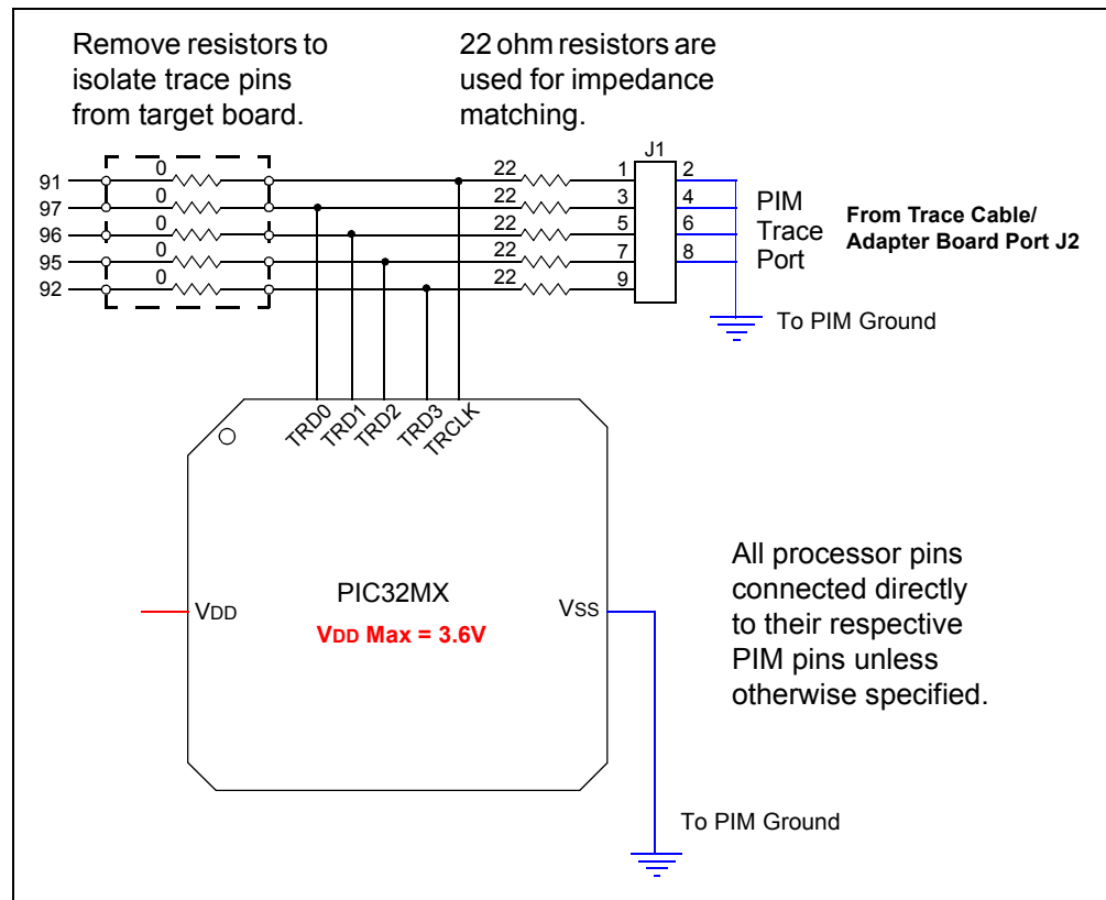
FIGURE 16-2: PIC32 PIM PIN CONNECTION DIAGRAM
