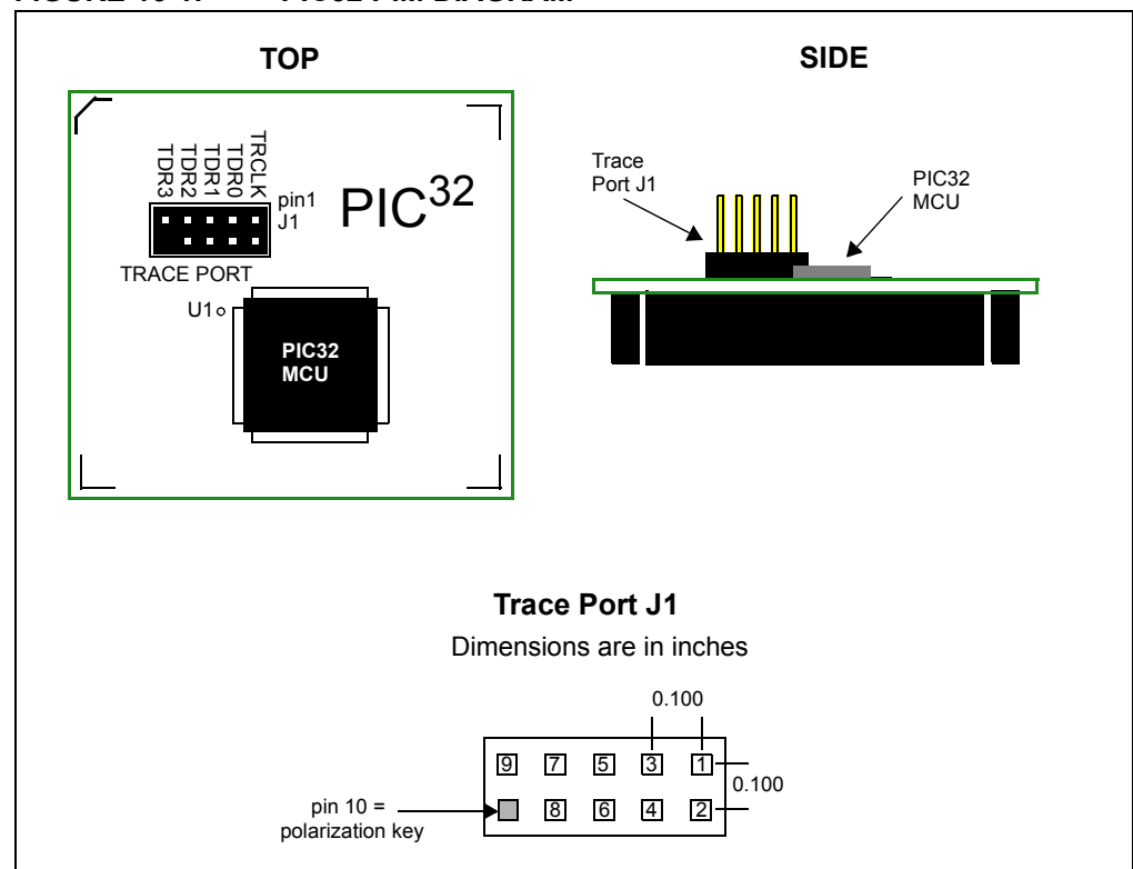
FIGURE 16-1: PIC32 PIM DIAGRAM
